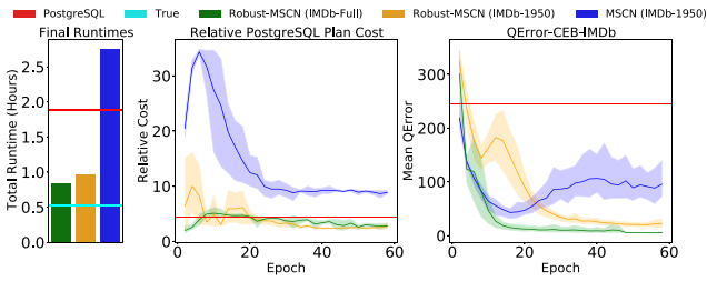
Figure 14: Final runtimes, and learning curves for models evaluated on the data drift scenario.
