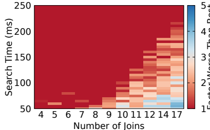
(b) After training, we plot the average query performance normalized to the best seen performance based on the number of joins in a query and the time spent in search. For queries with \leq 9 joins, the best seen performance is achieved with only 100ms of search time. Queries with more joins needed up to 230ms of search time.
