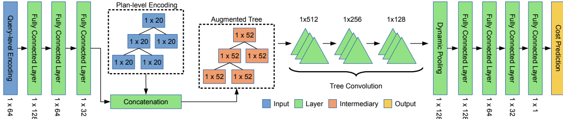
Figure 5: Value network architecture
