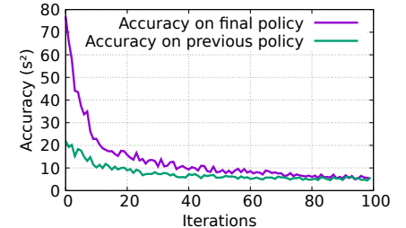
(c) Accuracy (MSE) of the value network per training iteration. Blue shows the accuracy of the value network at iteration i (x-axis) at predicting the latency of plans produced at iteration 100. Green shows the accuracy of the value network at iteration i at predicting the latency of plans produced at the previous iteration (iteration i - 1 ).
