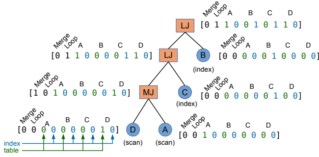
Figure 4: Plan-level encoding
